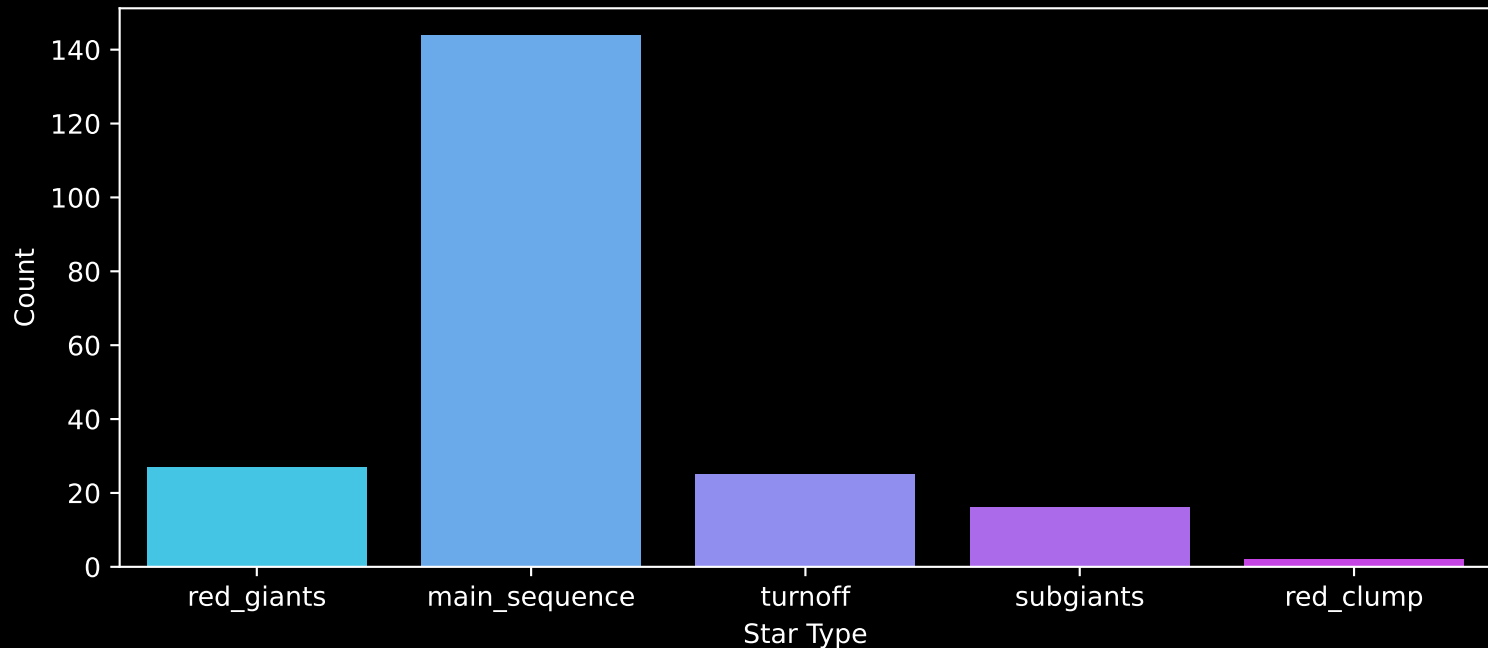
APOGEE DR17 Field: [K2_C14_244+55] Count plot of Star Type
