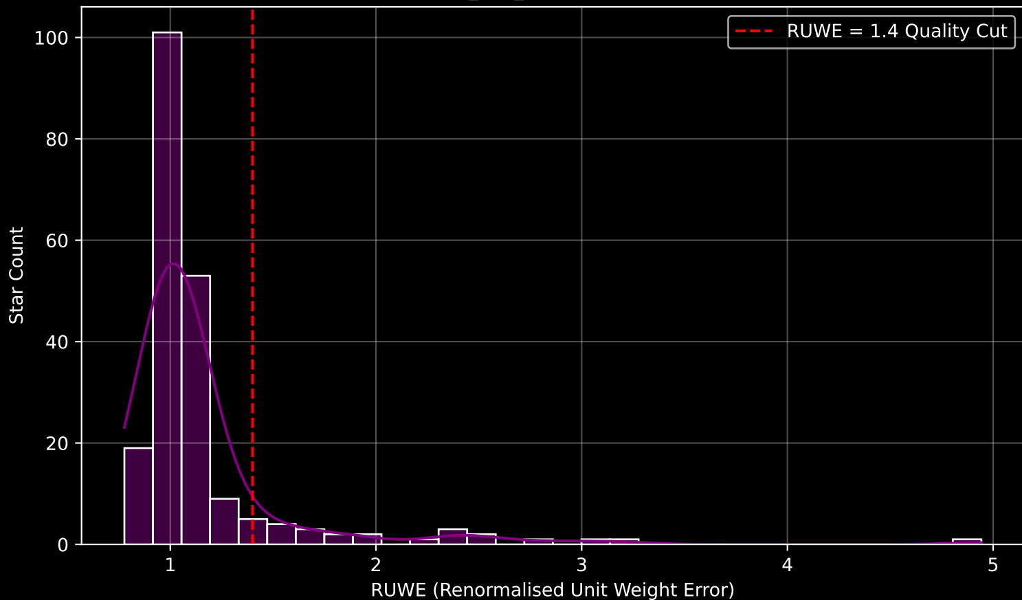
GAPOGEE DR17 Field [K2_C14_244+55] RUWE Distribution (n= 208)
