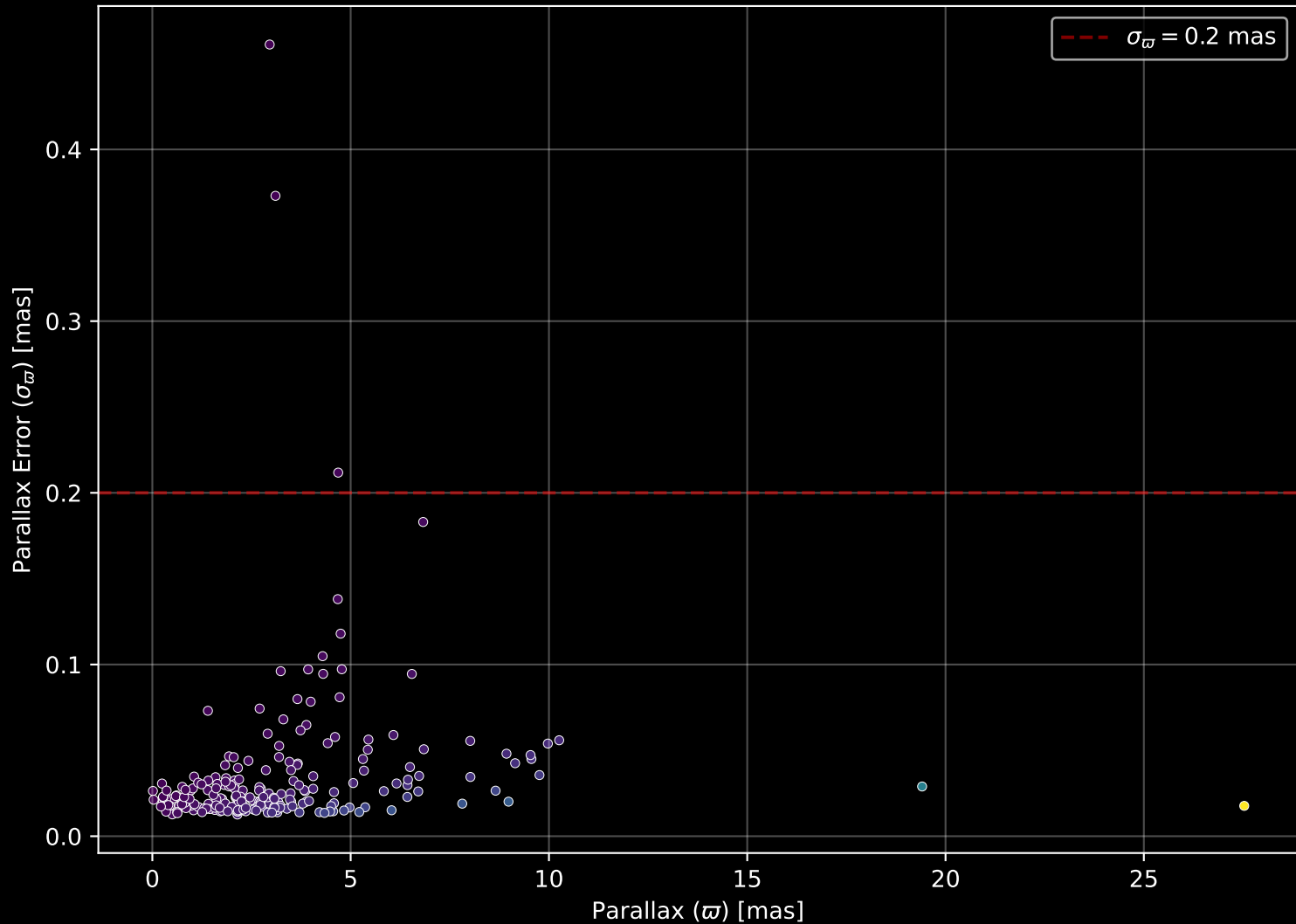
APOGEE DR17 Field: [K2_C14_244+55] Parallax Quality (n= 214)
