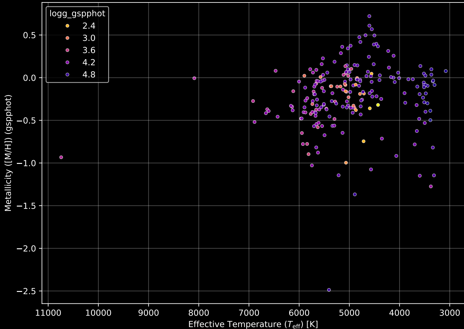
APOGEE DR17 Field: [K2_C14_244+55] Stellar Population Parameters (n= 214)
