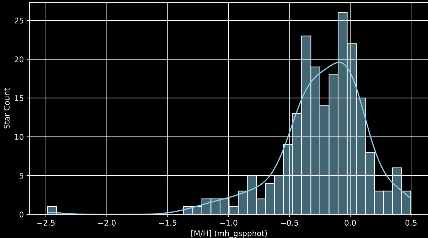
APOGEE DR17 Field: [K2_C14_244+55 [M/H] (mh_gspphot) (n= 211)
