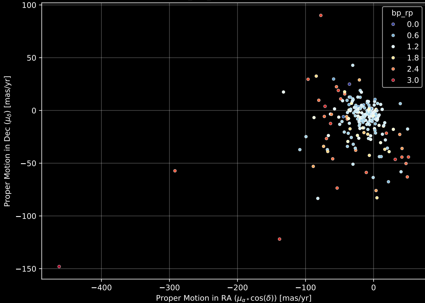
APOGEE DR17 Field: [K2_C14_244+55] Proper Motion Diagram (n= 214)
